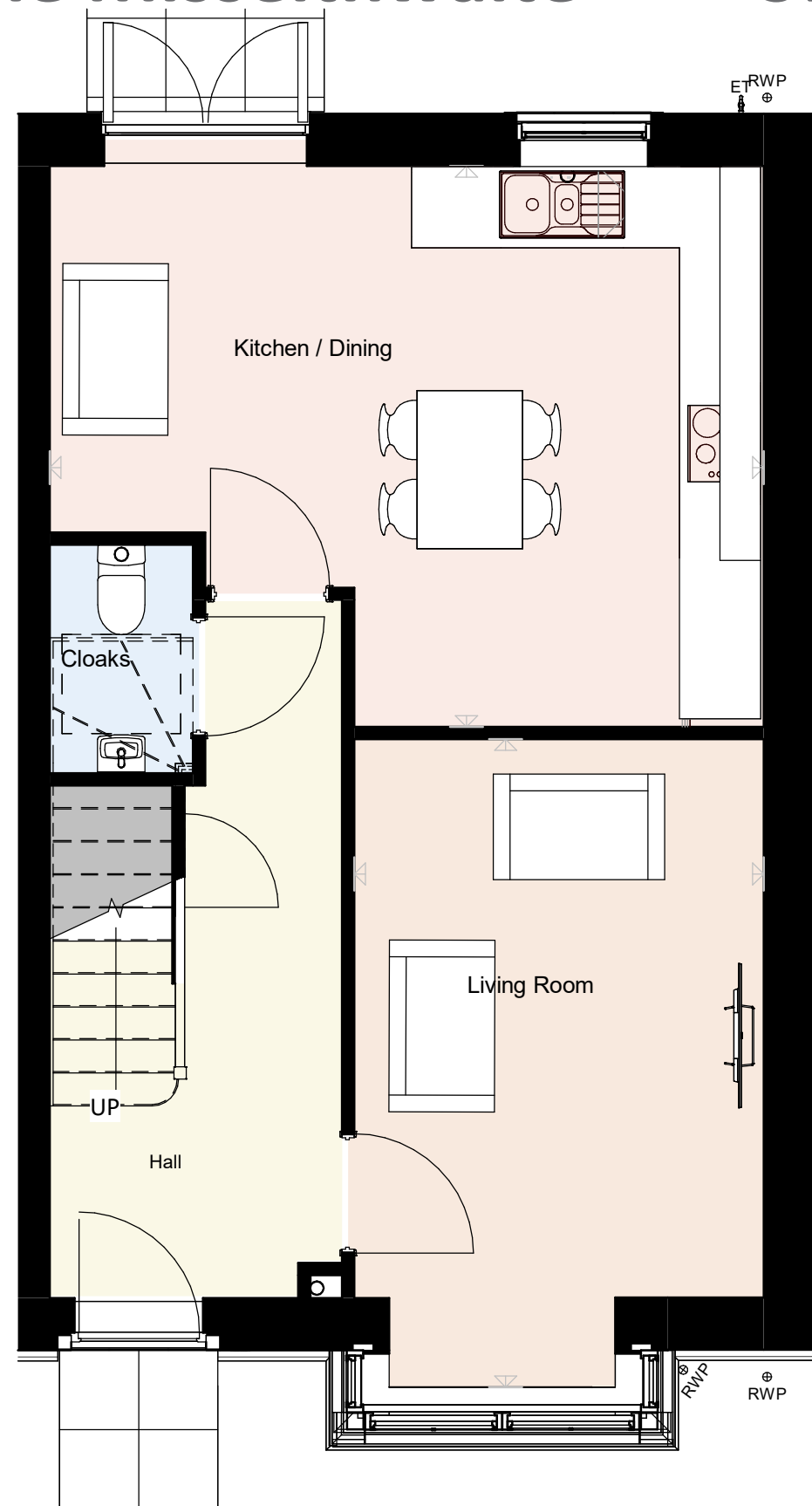
1 GROUND FLOOR SALES PLAN THE MISSELTHWAITE 1 : 50
